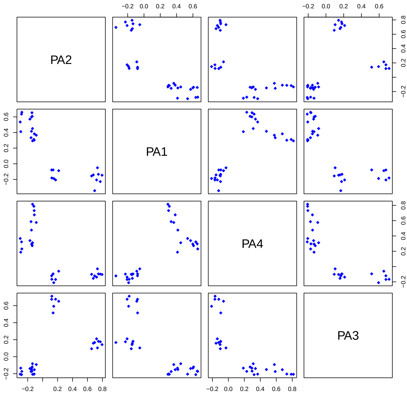
Varimax Loadings Matrix (All 4 Dimensions)
